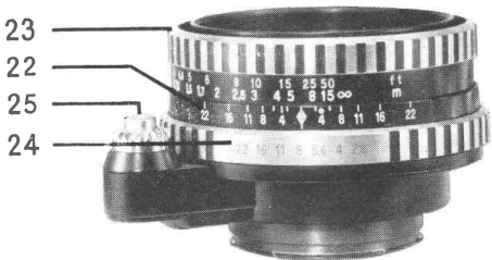
Automatic diaphragm mechanism disengaged
