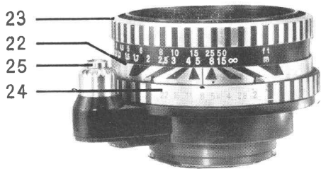
Automatic diaphragm mechanism engaged
