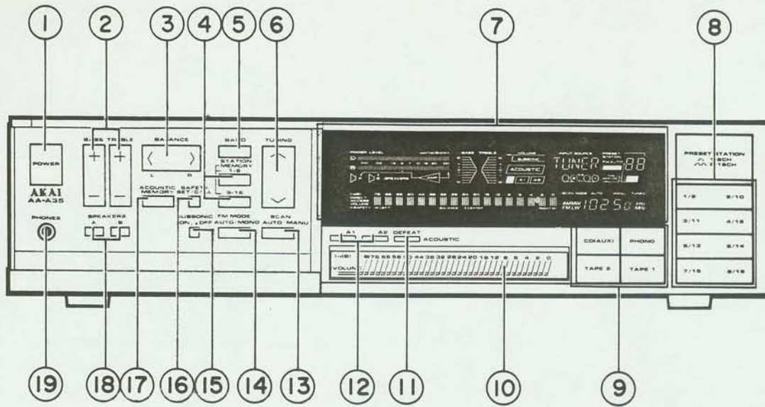
Fig. 3-1 Front View
