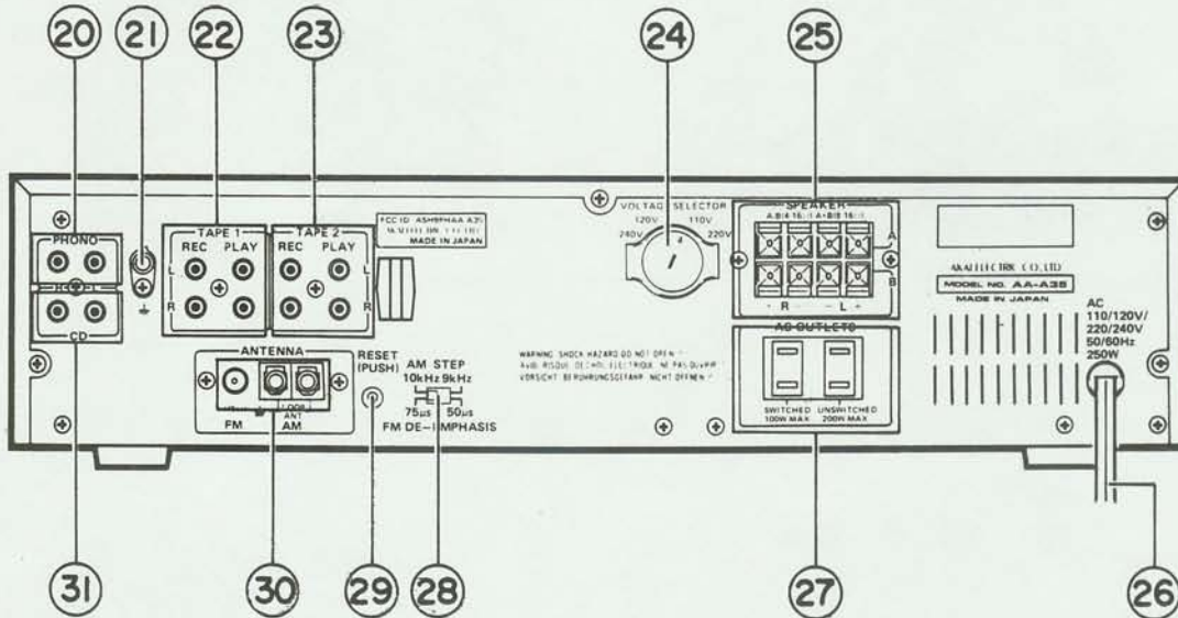
Fig. 3-2 Rear View
