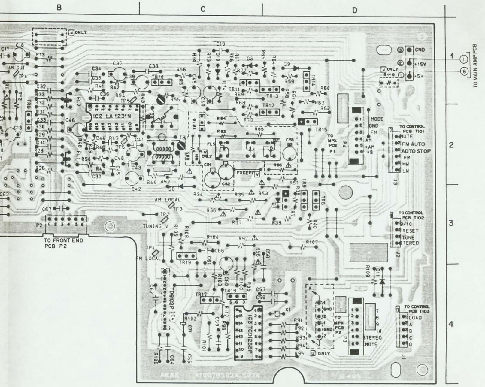
TUNER PCB A1007B502A U C A E V S
