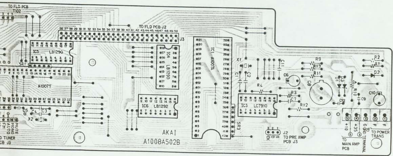
CONTROL PCB A1008A502B
