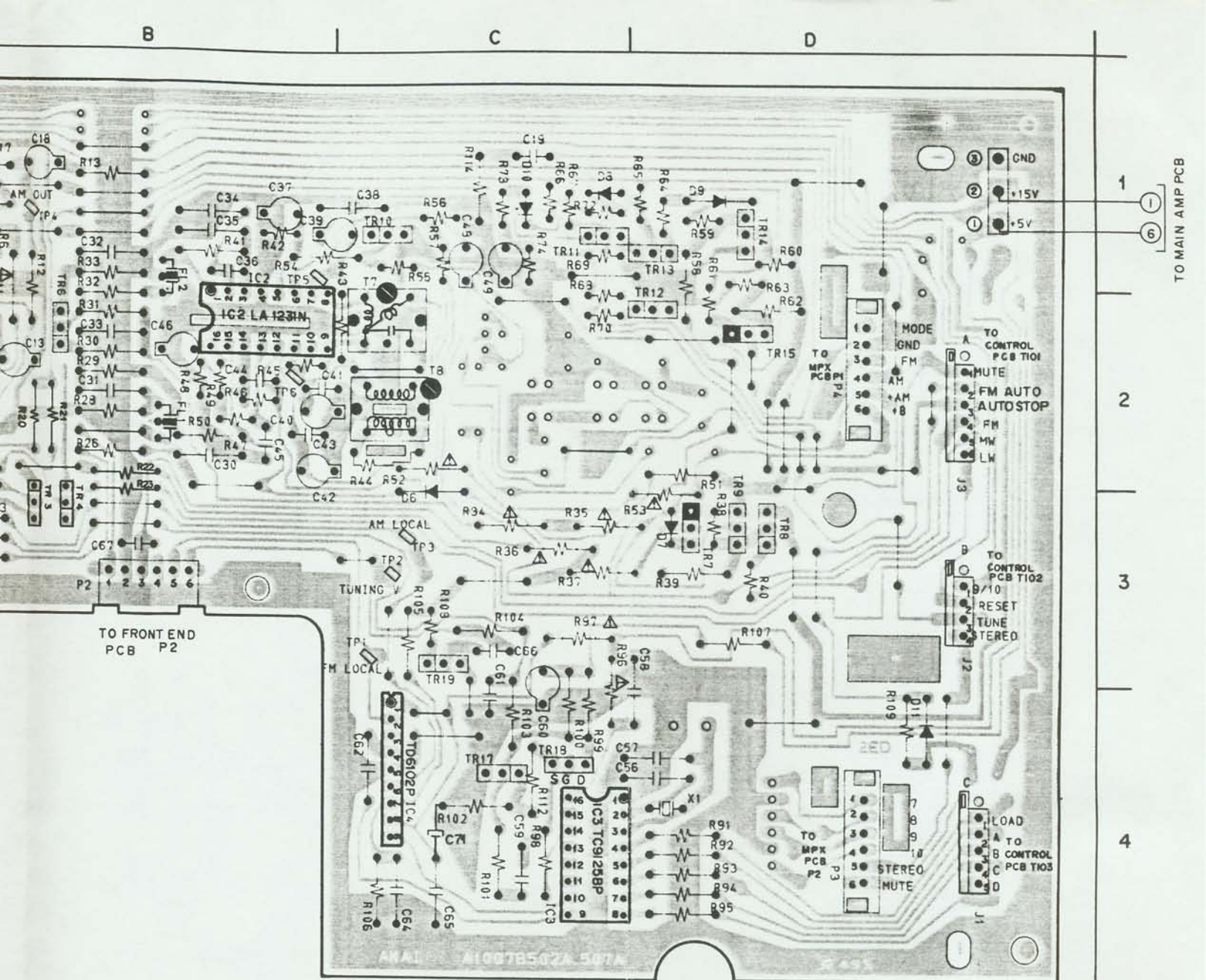
TUNER PCB A1007B507A (2ED) B E
