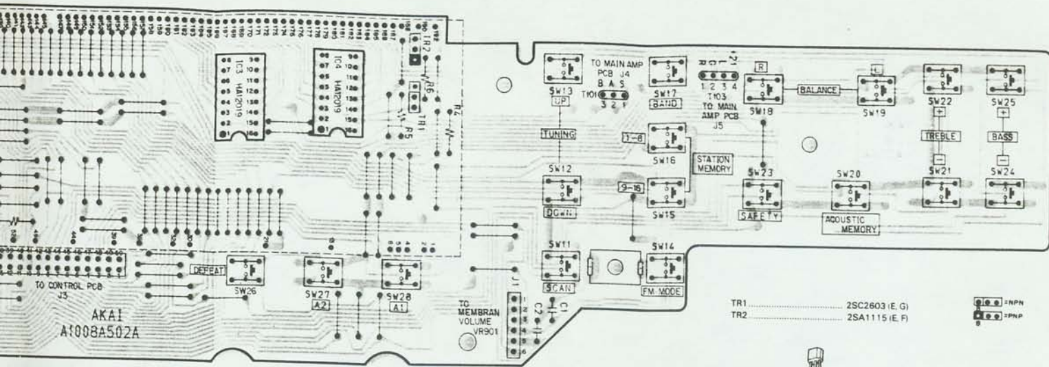
FLD PCB A1008A502A
