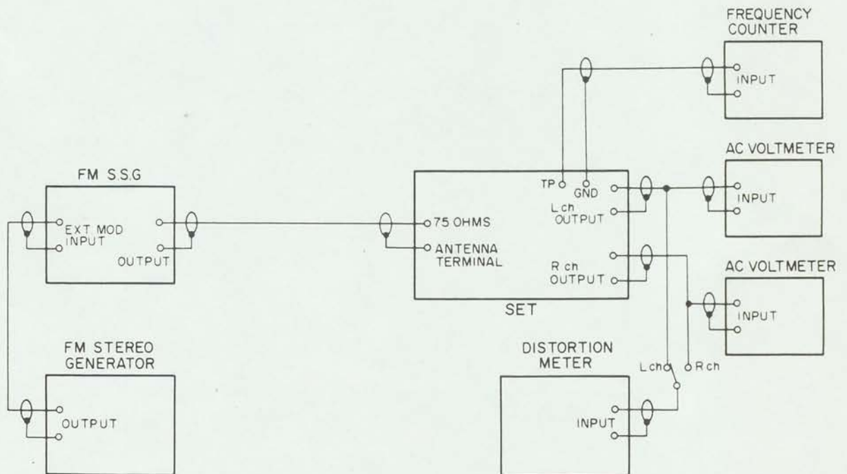
Fig. 7-2 Instrument Connections for FM Section Adjustment
