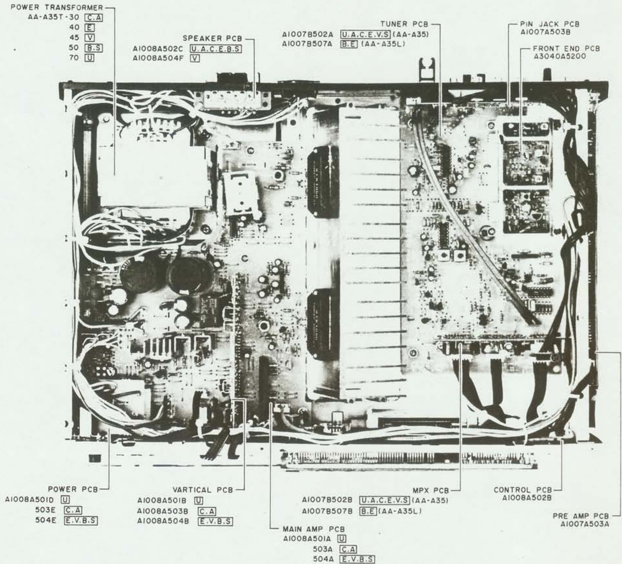
Fig. 4-2 Top View
