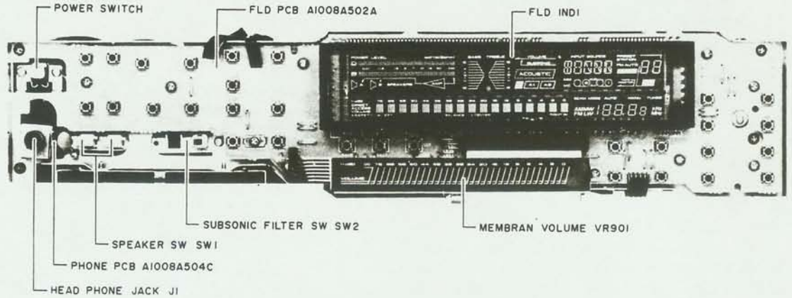
Fig. 4-1 Front View
