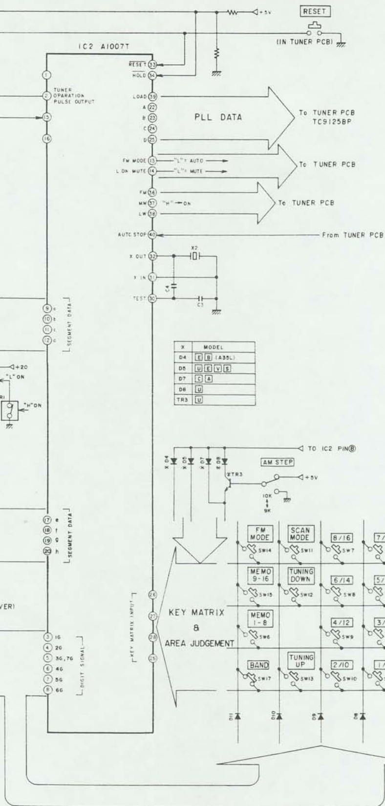
AA-A35/L CONTROL BLOCK DIAGRAM NO.2-1 84060IA
