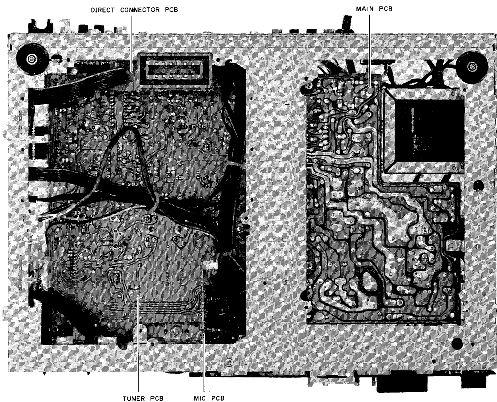
Fig. 4-2 Bottom View
