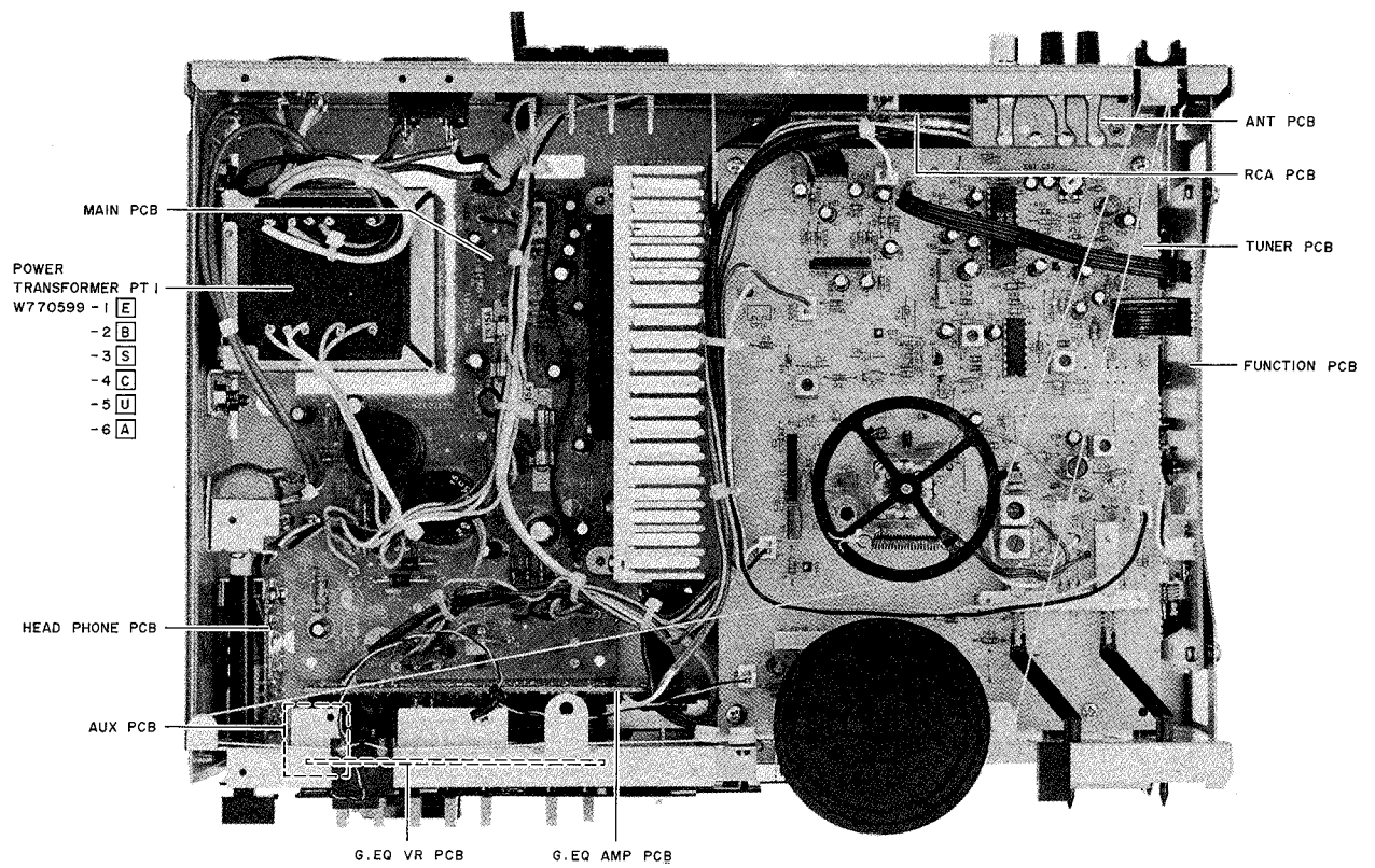
Fig. 4-1 Top View
