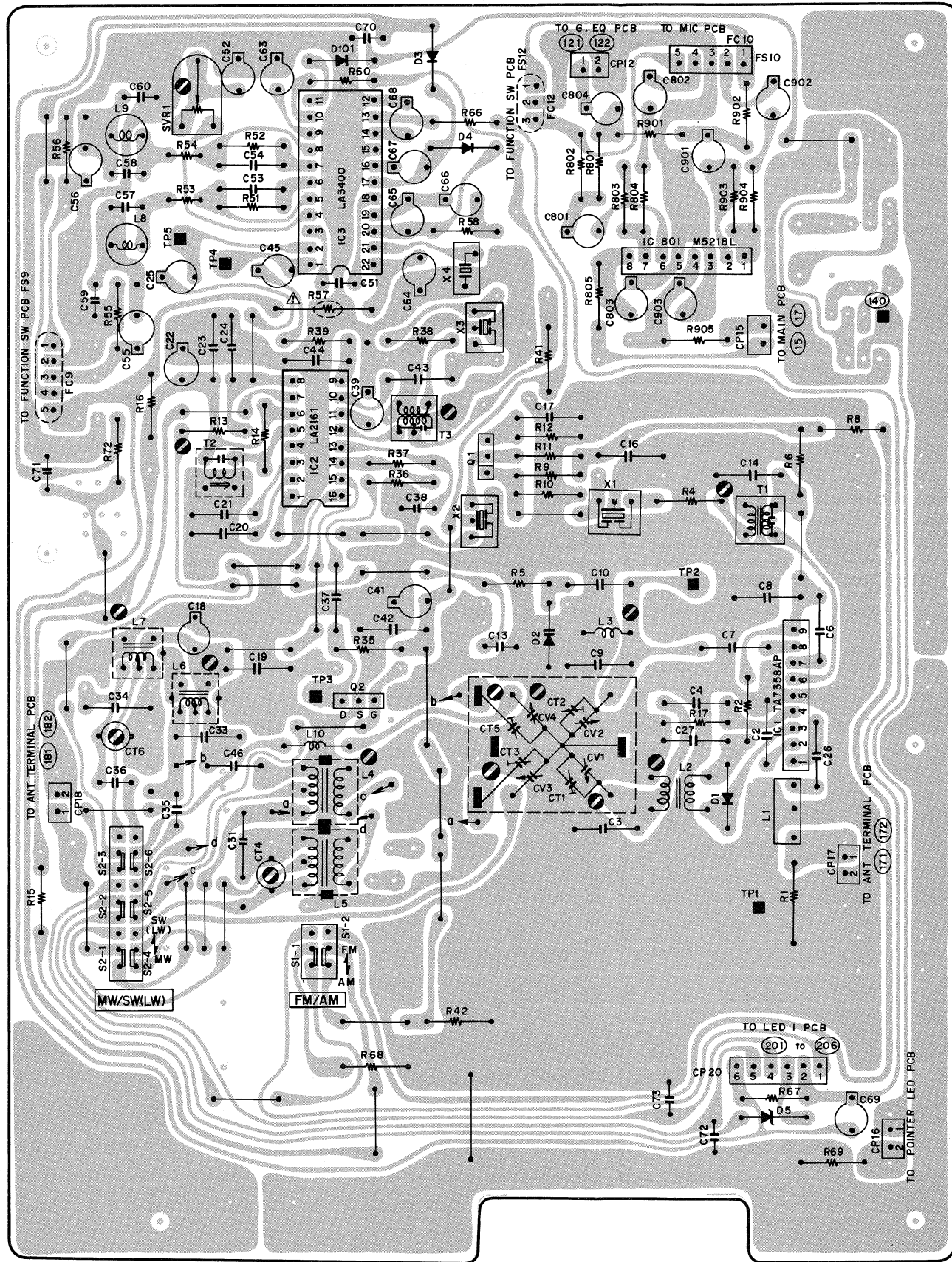
TUNER PCB
