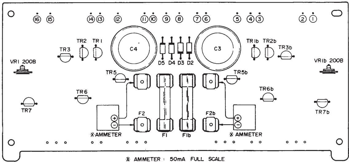
Fig. 4 Main Amp P.C Board M2-218
