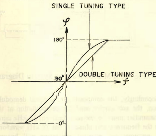
Fig. 7 Tuning Curve
