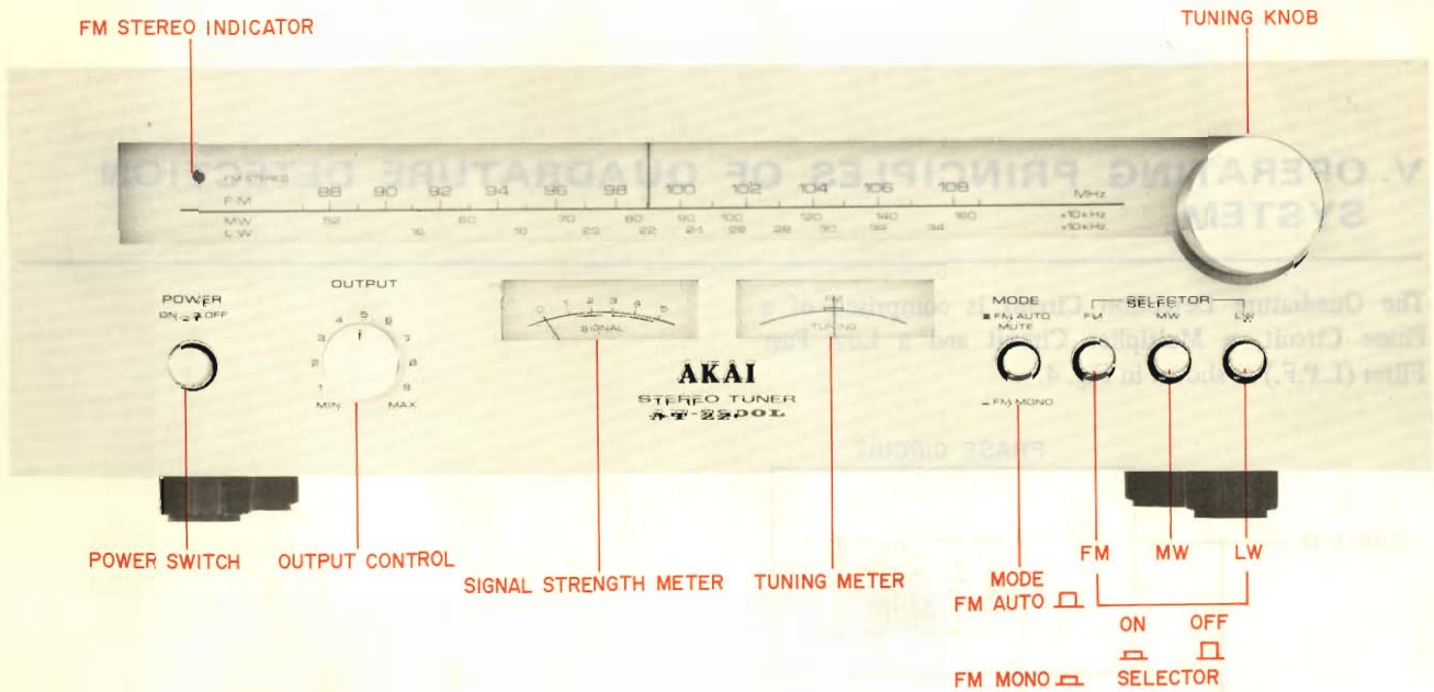
Fig. 2 Controls
