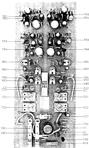
FIG. 15 PHOTO OF REC. AMP. P.C. BOARD (ND-5038)
