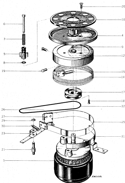
FIG. 3 ILLUSTRATION OF REEL MOTOR/REEL TABLE BLOCK
