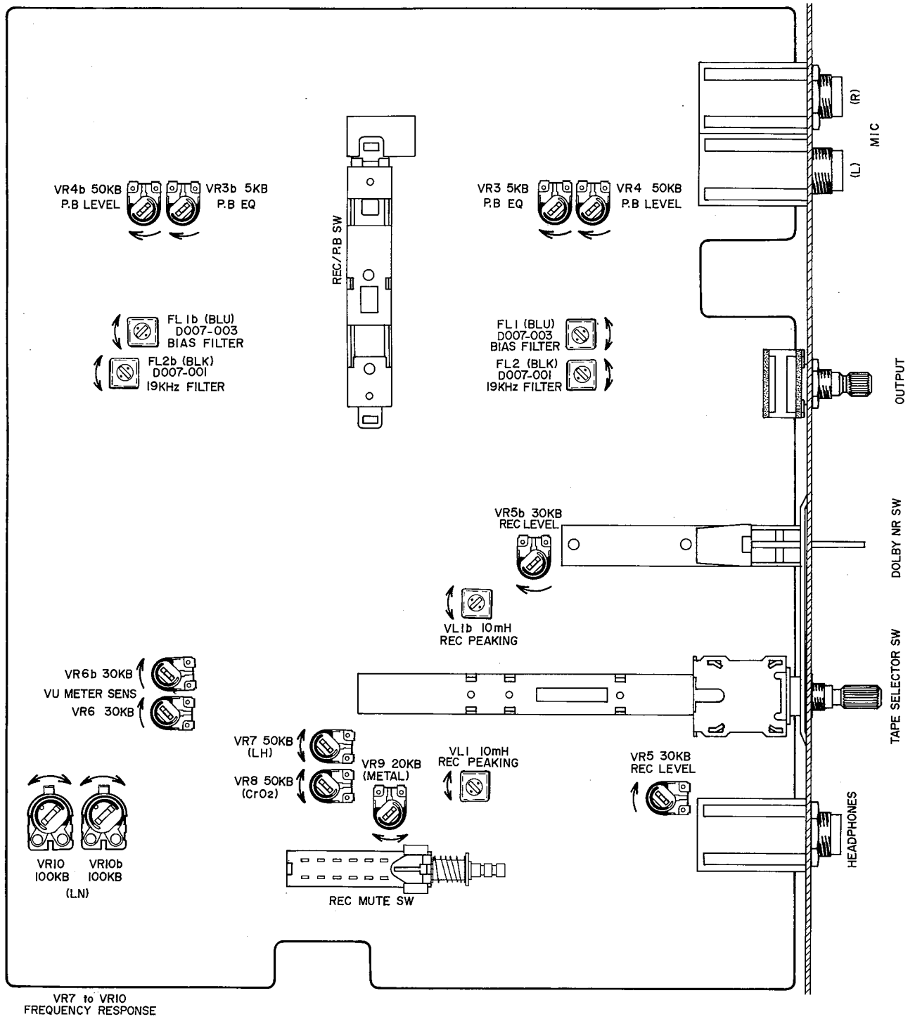
Fig. 25 Pre Amp P.C Board CE-5201A
