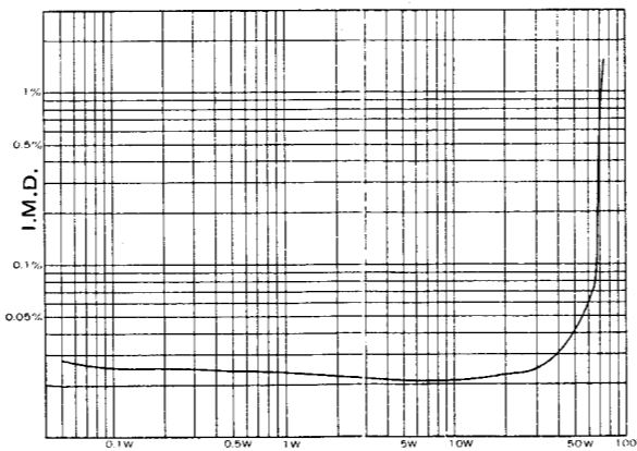
INTER-MODULATION DISTORTION Input; Main in, Frequency and Modulation Ratio 70Hz; 7KHz±4 : 1
