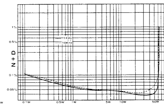
NOISE + HARMONIC DISTORTION Input; Main in, 8Ω load, incl. oscillator distortion 0.03%
