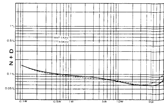
NOISE + HARMONIC DISTORTION Input; Main in, 4Ω load, incl. oscillator distortion 0.03%
