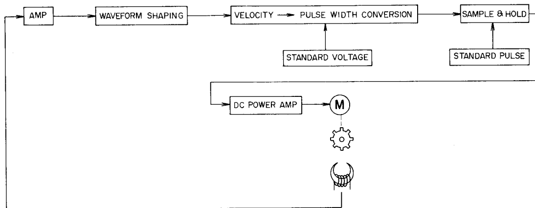
Fig. 5 Block Diagram
